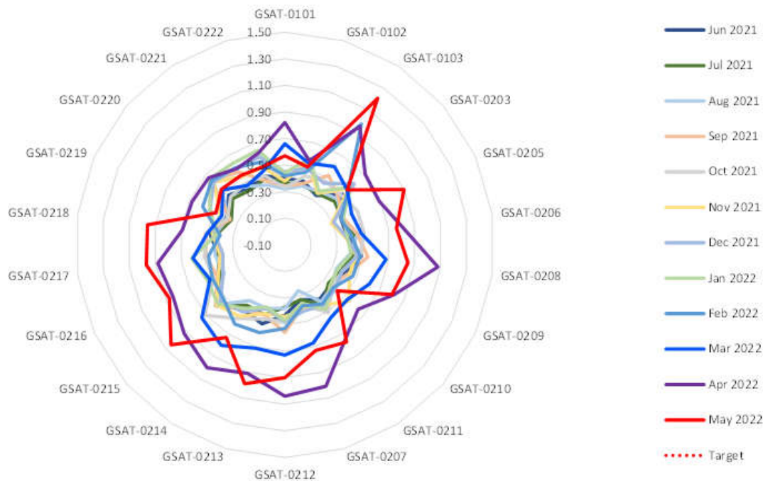
Single Frequency Ranging Accuracy [m] - Worst Case of monthly 95%
