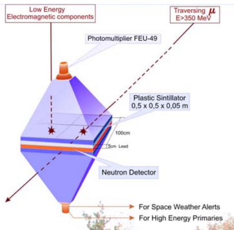
Figure 9. Schematic diagram of the new detector for muons and neutrons installed at the Aragats Space Environmental Center, Armenia (courtesy: A. Chilingarian).
