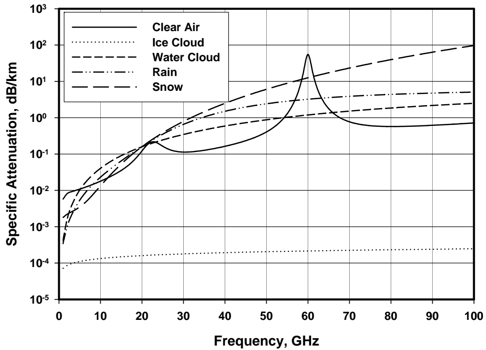
Figure (5): Specific attenuation due to different atmospheric constituents as a function of radio frequency and atmospheric pressure for P= 1013.25 \text{ hPa} , T=293^\circ \text{ K} and \rho_v = 7.75 \text{ g/m}^3 .
