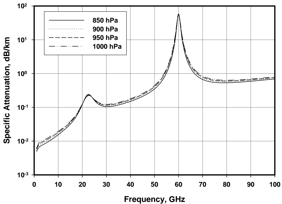
Figure (4): Specific attenuation due to atmospheric gases as a function of radio frequency and atmospheric pressure for T=293^\circ K and
