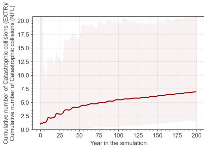
Figure 26 Cumulative number of catastrophic collisions in LEO in the simulated scenarios of long-term evolution of the environment.
