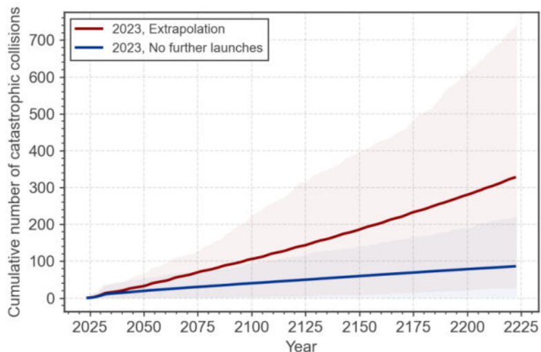
Figure 24 Cumulative number of catastrophic collisions in LEO in the simulated scenarios of long-term evolution of the environment.
